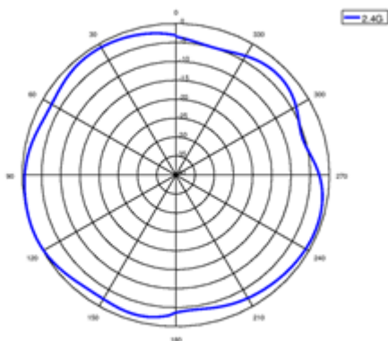
2.4G (Horizontal)
